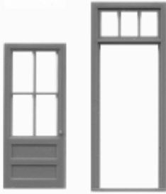
4 LITE DOOR/TRANSOM 39" W x 92" H .5" x 1.35" OPENING
